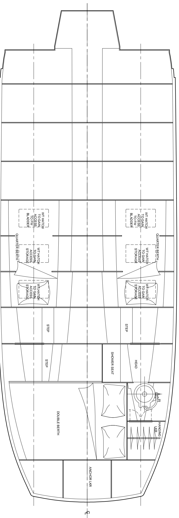
1 VIEW : SHOWING PLAN VIEW OF LOWER ACCOMMODATIONS Scale: 1:15
